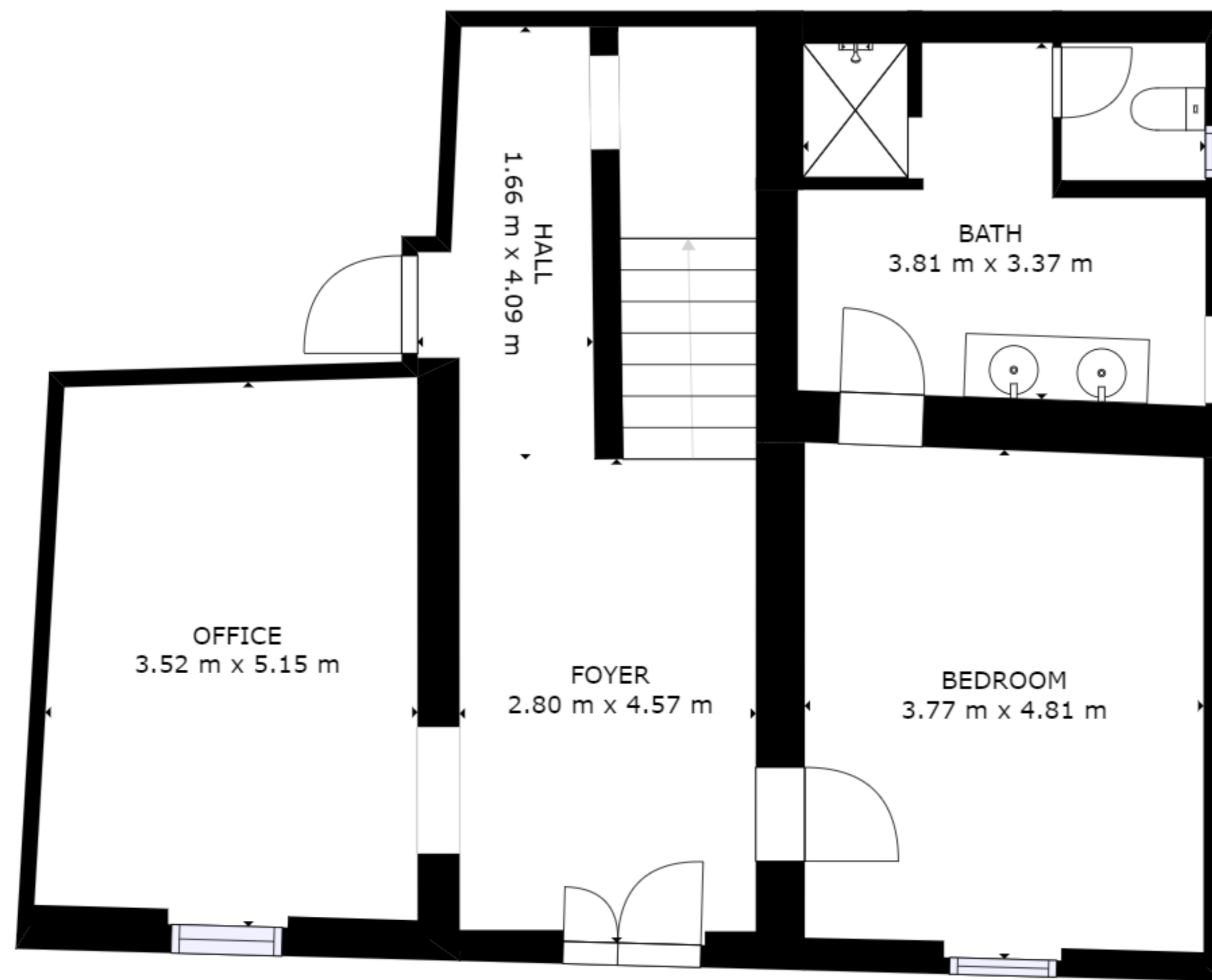
FLOOR 1
